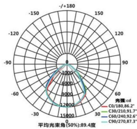
Light Distribution Diagram
